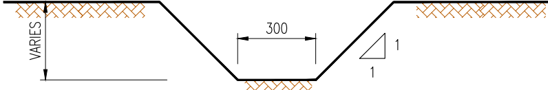
TEMPORARY EARTH DRAIN DURING CONSTRUCTION SCALE 1:20
