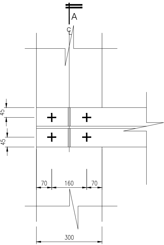
DETAIL '1' SCALE : 1:10
