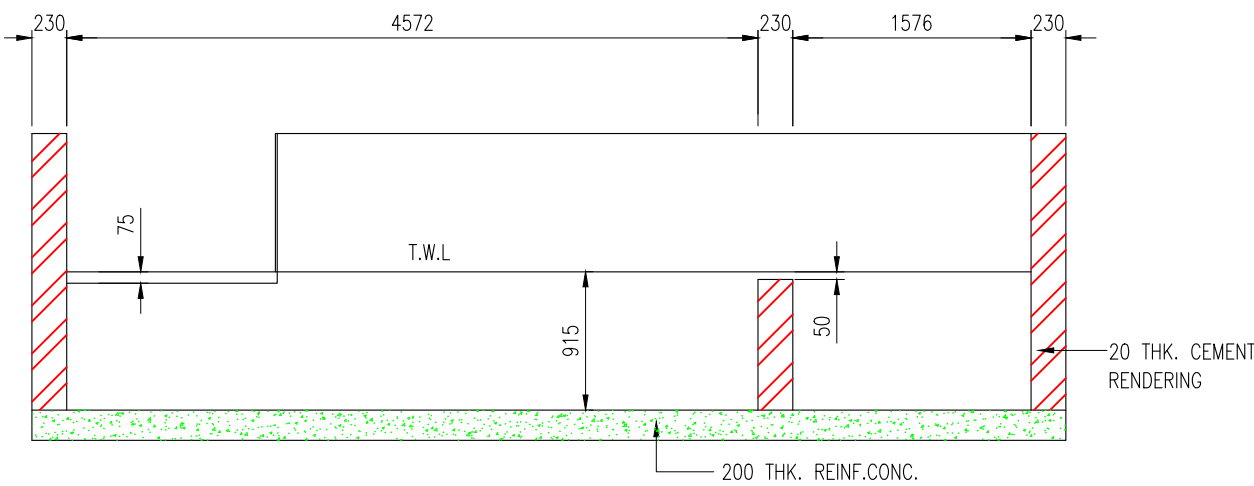
SECTION C - C SCALE 1:50
