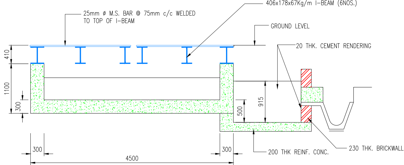
CROSS SECTION (X-X) SCALE 1:50
